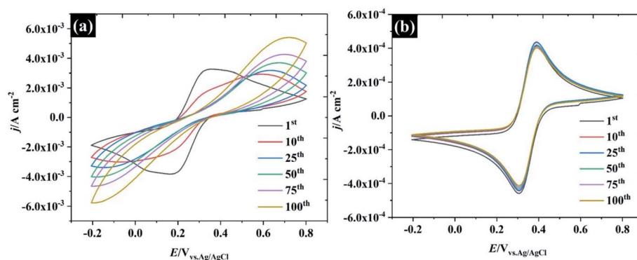
Fig. 6 Repeated CV cycles at 100 \text{ mV s}^{-1} at HOPG in 10 mM \text{K}_3\text{Fe(CN)}_6 using (a) 0.5 M KF, and (b) 17 M KF as supporting electrolytes.
