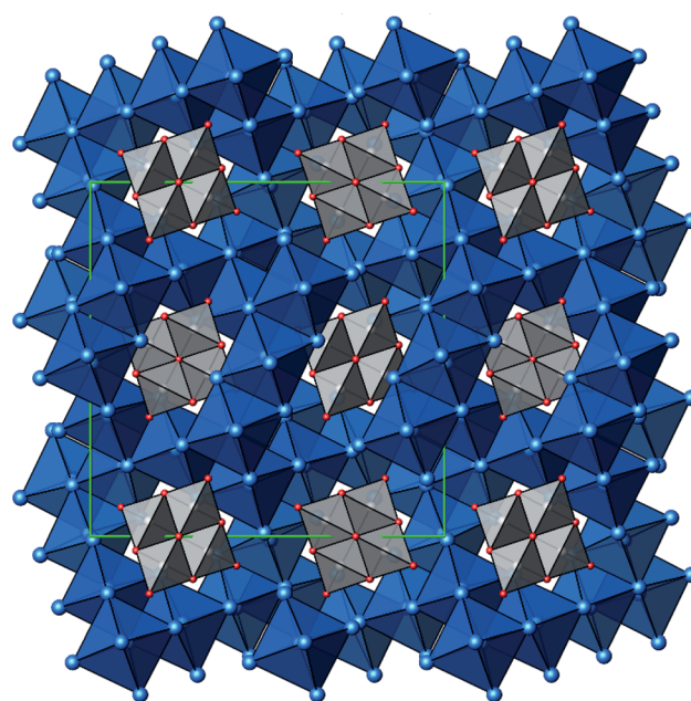
Fig. 3 Projection of the crystal structure of \text{Ag}_{16}\text{B}_4\text{O}_{10} , view along [001] , with margins of the unit cell (green). Color code: Ag (blue spheres), B (grey spheres), O (red spheres), blue octahedra ( \text{Ag}_6 ), grey tetrahedra ( \text{BO}_4 ).
