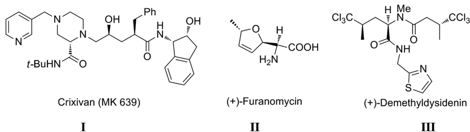
Fig. 1 Structure of Crixivan I, furanomycin II and demethylsidsidenin III.
