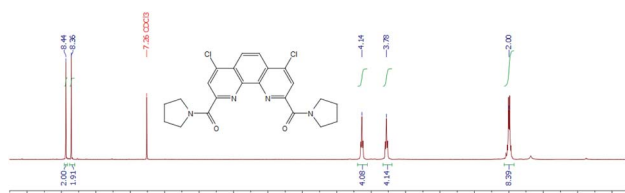
Fig. 9 1 H NMR spectrum of 3a in CDCl 3 at 25 °C.
