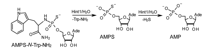
Scheme 3 The HINT1 catalyzed hydrolysis of adenosine-5'- O -(( L -tryptophan amide- N_{\alpha} -yl)-phosphoramidothioate) (AMPS-Trp-NH 2 ), followed by desulfuration of the AMPS intermediate leading to the formation of adenosine-5'- O -phosphate.
