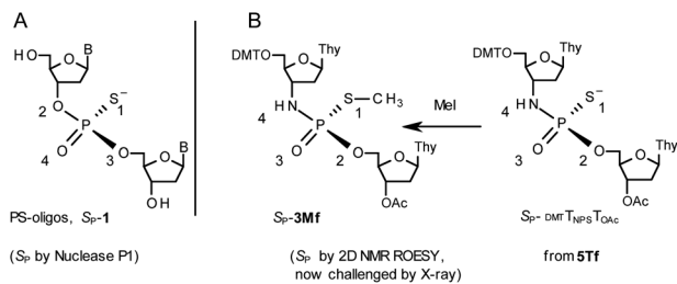
Chart 3 Orientation of the sulfur, phosphoryl oxygen and thymidine O5' atoms around the phosphorus atoms: Panel A, in phosphorothioate S_P -1, ref. 23; Panel B, 2D NMR ROESY based assignment (here challenged by X-ray analysis of 10f , Scheme 1) in the S -methylated S_P - 3Mf , ref. 22 (the phosphoramidothioate diester precursor was obtained from fast-eluting 5Tf ). The Arabic numerals 1–4 indicate the priority of substituents around the phosphorus atoms according to the Cahn–Ingold–Prelog rules. Note: to establish the priority of substituents, the formal double bond between the phosphoryl oxygen atom and the phosphorus atom ( P=O ) should be considered a single one.
