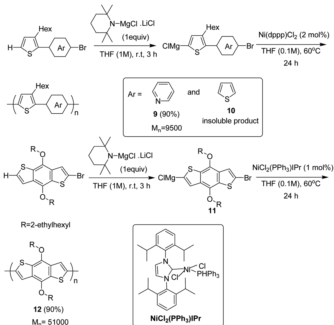
Scheme 6 Ni-catalyzed synthesis of poly(thienylenepyridylene) 9 , poly(thienylenephénylene) 10 and poly(benzodithiophene) 12 .
