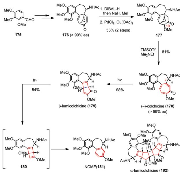
Scheme 25 4 \pi electrocyclization in the total synthesis of colchicine derivatives.
