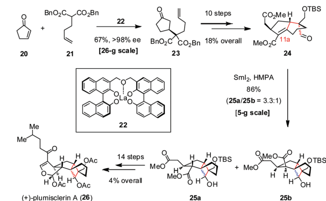
Scheme 4 Ketyl-olefin radical cyclization in the total synthesis of (+)-plumisclerin A.
