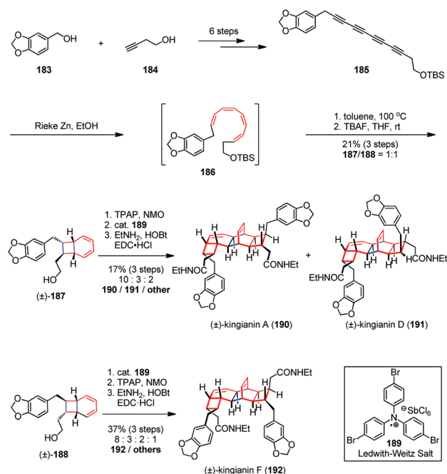
Scheme 26 8 \pi -6 \pi electrocyclization cascade in the total synthesis of kingianins.
