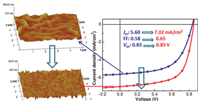
Fig. 7 Influences of surface roughness of the ZnO electron transport layer on the photovoltaic performance of organic inverted solar cells. Reproduced with permission. 113 Copyright 2012, American Chemical Society.
