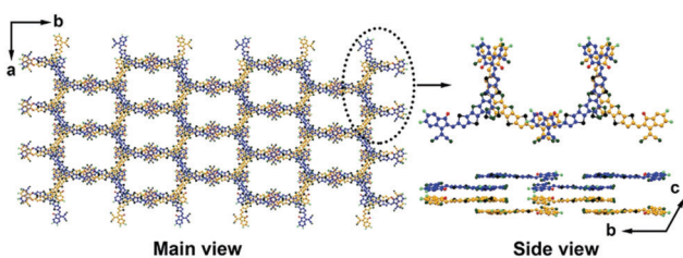
Fig. 5 Molecular packing sketch map of Y6 according to single crystal data (the alkyl chains were omitted for clarity). Reproduced with permission. 74 Copyright 2020, Wiley-VCH.
