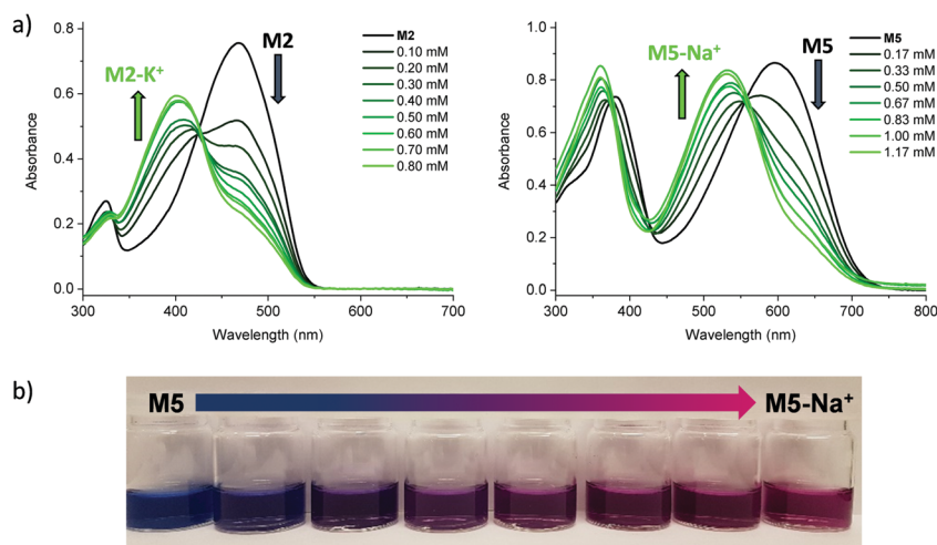
Fig. 2 (a) Representative UV-vis absorption spectra in tetrahydrofuran solution for M2 upon titration with aliquots of 0.002 M KBPh 4 in tetrahydrofuran (left) and for M5 upon titration with aliquots of 0.005 M NaBPh 4 in tetrahydrofuran (right); (b) photographs of M5 titration series with NaBPh 4 in tetrahydrofuran. All data recorded at room temperature.
