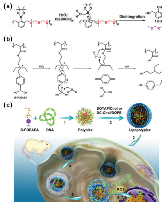
Fig. 53 (a and b) A positive-to-negative convention mechanism of surface charge for gene carriers. (c) Schematic representation of cationic-lipid-coated ROS-responsive polyplexes for gene delivery. Reprinted from ref. 395, 396 and 399 with permission. Copyright (2017, 2016, and 2018) from Wiley-VCH and American Chemical Society.
