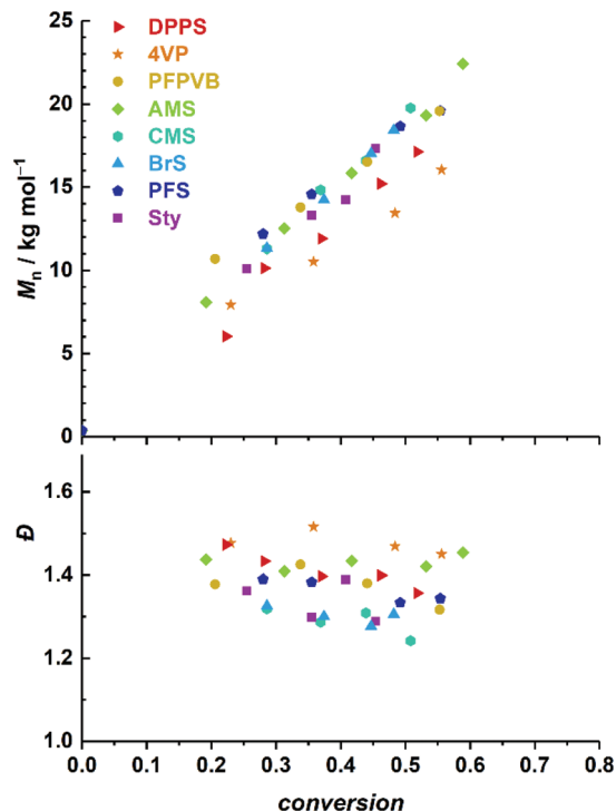
Fig. 2 Evolution of number-average molar mass (top) and dispersity (bottom) with MMA conversion for the SG1-mediated polymerization of MMA in toluene at 80 °C, in the presence of 5 mol% of various styrenics.
