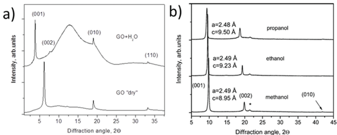
Fig. 5 Examples of XRD patterns recorded from graphite oxide powder (synthesized using the Brodie method) in liquid solvents: (a) synchrotron radiation ( \lambda = 0.71170 Å) XRD recorded in transmission mode under ambient air conditions from water filled sealed glass capillaries 111 (b) XRD patterns recorded using a standard diffractometer with CuK \alpha radiation in reflection mode. 112 The samples are immersed in liquid alcohols and sealed using plastic foil (the peak marked by * is from the foil).
