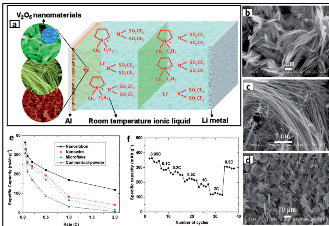
Fig. 15 (a) Schematic representation of a lithium metal battery using V 2 O 5 nanomaterials and room temperature ionic liquid electrolyte. SEM images of diverse morphologies of V 2 O 5 materials: (b) nanoribbons (c) nanowires (d) microflakes and their corresponding (e) specific capacities; (f) cycle life of V 2 O 5 nanoribbon. "Adapted with permission from ref. 218. Copyright (2008) American Chemical Society."
