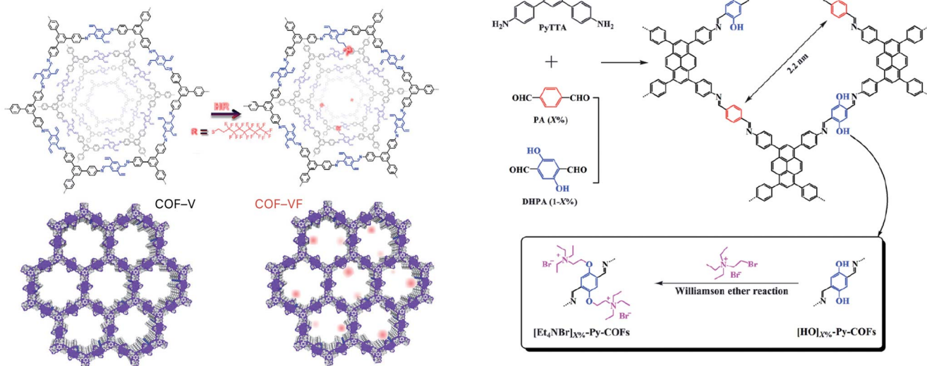
Fig. 46 Williamson ether synthesis of IL-functionalized [\text{Et}_4\text{NBr}]_{X\%}\text{-Py-COFs} for catalyzing the formylation reaction. Adapted with permission. 305 Copyright 2016, The Royal Society of Chemistry.
