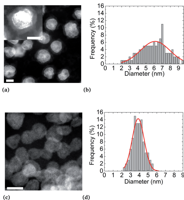
Fig. 4 STEM-HAADF micrographies and size distribution histograms of Ni 3 Pt NPs elaborated at (a and b) 200 ^\circ\text{C} showing a core–shell structure and an observable organic layer surrounding the particle in the magnified image in the inset and at (c and d) 280 ^\circ\text{C} showing alloyed particles (scale bar = 5 nm).
