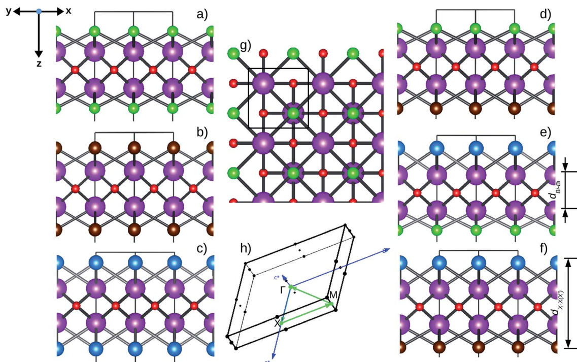
Fig. 1 Optimized crystal structures of pristine BiOX (left panels a, b, c) and Janus BiOX 0.5 X' 0.5 (right panels d, e, f) monolayers in side view. The conventional tetragonal unit cell is used for all calculations, as marked with the black solid box. The top view is shown only for one case, i.e. the BiOCl monolayer (panel g). The high symmetry k -path is indicated with the green colored solid line in the first Brillouin zone (panel h) for the chosen case of the BiOCl monolayer, and was obtained using the Xcrysden tool. In the structure plots, the large violet colored balls correspond to the Bi atoms, the small red colored balls are the O atoms, and the medium sized green, brown, and blue colored balls are the Cl, Br, and I atoms, respectively, and the plots were obtained with the VESTA crystal structure visualization tool. 16 The width of the ML, d_{X-X(X')} , and the inner (Bi 2 O 2 ) 2+ laminar width, d_{Bi-Bi} , are marked with double headed arrows.
