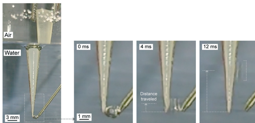
Fig. 22 Optical images of underwater air bubbles traveling on cones with various orientations (adapted from ref. 19).
