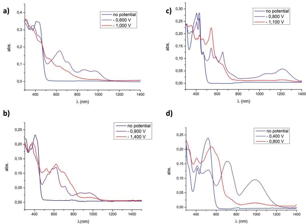
Fig. 5 Absorption spectra measured upon electrochemical reduction of (a) 4a [OTf] 2 , (b) 4b [OTf] 2 (c) 6 [OTf] 2 , and (d) 8 [OTf] 2 ( c = 5 \times 10^{-4} M) in DCM (0.2 M Bu 4 NPF 6 ).
