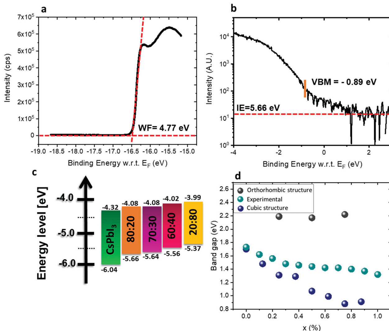
Fig. 5 (a) Photoemission cut-off measured via UPS for \text{CsSn}_{0.2}\text{Pb}_{0.8}\text{I}_{2.6}\text{Br}_{0.4} . (b) The position of the VBM and ionization energy (IE) for \text{CsSn}_{0.2}\text{Pb}_{0.8}\text{I}_{2.6}\text{Br}_{0.4} measured by UPS. (c) Energy diagram of the different materials used in this study. The band gap of \text{CsPbI}_3 is relatively wide with respect to the literature value, 62 which is due to degradation as discussed in the text. (d) Experimental results and theoretical calculation of the band gaps for the various ratios when adding \text{SnBr}_2 . x represents the ratio Pb : Sn.
