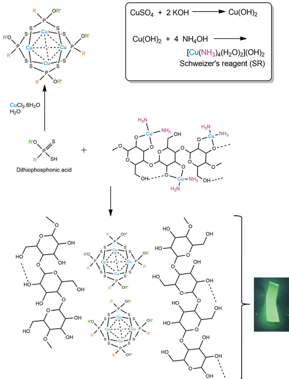
Scheme 1 Formation of a tetranuclear copper(I) cluster from \text{Cu}(\text{II}) and dithiophosphonic acid precursor (top left). Inset: Key steps in the formation of Schweizer's Reagent. Bottom: Luminescent cellulose/ \text{Cu}_4\text{L}_4 paper formed from the direct reaction between dithiophosphonic acid and a \text{Cu}(\text{II}) precursor present in SR.
