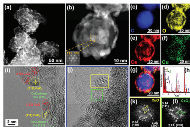
Fig. 2 (a and b) HAADF-STEM images of CuO–CeO 2 /CB. The inset in image (b) shows the corresponding FFT of CuO–CeO 2 /CB. EDS elemental maps of (c) C, (d) O, (e) Ce, (f) Cu, and (g) overlay of C (blue), Ce (red), and Cu (green) over the region shown in image (b), along with corresponding EDS spectrum (h). (i) HRTEM image of CuO–CeO 2 /CB. (j–l) Magnified image of the blue rectangle in image (i) and FFTs of the regions enclosed by the yellow and green rectangles in image (j).
