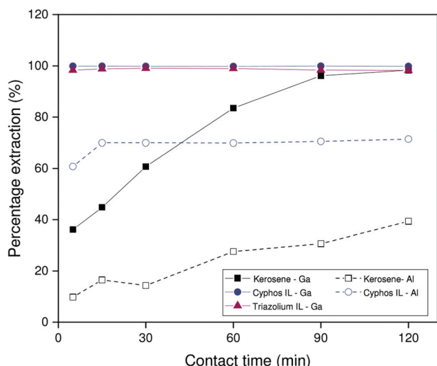
Fig. 5 Percentage extraction as a function of time for 200 ppm solutions extracted from 1.700 mol L -1 sodium carbonate by 5 vol% Kelex® 100 in [EhEhT 23 ] 2 [SO 4 ], 5 vol% Kelex® 100 in [C101] 2 [SO 4 ] and 5 vol% Kelex® 100 in kerosene modified with 10 vol% 1-decanol. Phase ratio: 1 : 1 organic to aqueous. The HLE procedure was followed for [EhEhT 23 ] 2 [SO 4 ].
