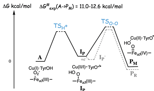
Fig. 7 Sketch of the energy profile for the suggested two step mechanism for the O–O bond cleavage in A and B family CcOs. Starting from the observed compound A with molecular oxygen bound to the high-spin heme a_3 a proton is transferred from the active site tyrosine, together with an electron, to form the hydroperoxo intermediate labeled I P . The electron is taken either from the tyrosine or from \text{Cu}_B . In the mixed-valence enzyme the O–O bond is cleaved forming the observed P M intermediate. In the fully reduced enzyme an electron is transferred from the low-spin heme forming I P − with a tyrosinate, from which the O–O bond cleavage yields the observed P R intermediate, with a tyrosinate.
