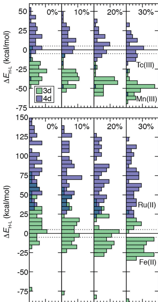
Fig. 7 Normalized histograms of \Delta E_{H-L} (in \text{kcal mol}^{-1} ) (bin width: 5 \text{ kcal mol}^{-1} ) for 51 pairs of 3d Mn(III) and 4d Tc(III) TMCs (top) and 64 pairs of 3d Fe(II) and 4d Ru(II) TMCs (bottom). Histograms are filled translucent for 3d (green) and 4d (dark blue) TMCs to show regions of overlap. A zero line is indicated as black solid where HS–LS spin state ordering changes, and a range of 5 \text{ kcal mol}^{-1} around that line is indicated with black dotted lines. The panes correspond to increasing % HF exchange from left to right, as labeled in top inset.
