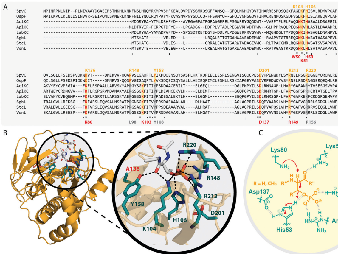
Fig. 6 (A) Excerpt of an alignment of OspF from Shigella dysenteriae and SpvC from Salmonella paratyphi with the lyase domains of exemplary class III (Ac1KC, Ap1KC, LabKC) and class IV (SgbL, StcL, VenL) lanthipeptide synthetases. Catalytic residues of the OspF protein family pThr lyases are highlighted in orange, catalytic residues of class III/IV lyase domains in red. Above the alignment, numbering of the catalytic residues of SpvC are shown. Below the alignment, numbering of the catalytic residues of VenL are shown. (B) Crystal structure of a K136A variant of SpvC (PDB code 2Q8Y) with bound substrate zoomed in on the active site. For clarity, only a fragment of the pThr-containing peptide substrate is shown. The K136 residue of WT SpvC acts as catalytic base during the \beta -elimination reaction. (C) Schematic showing the catalyzed phosphate elimination reaction with the hypothesized 12 functions for the catalytically important residues in VenL.
