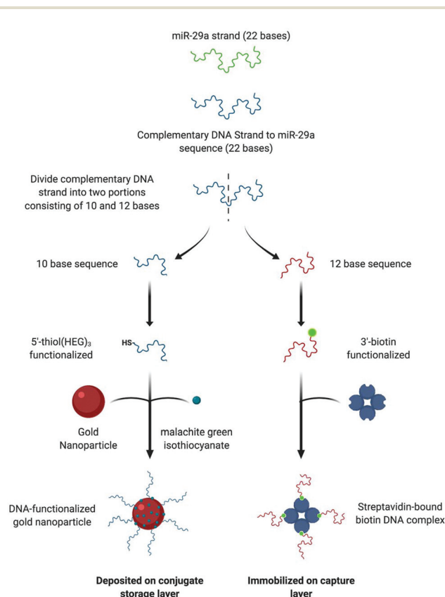
Fig. 1 The schematic shows how the components comprising the split-probe hybridization assay are designed. A 22 base DNA strand complementary to the miR-29a sequence is first developed, then divide the split into two portions consisting of 10 and 12 bases. The 10 base sequences is modified at the 5' end using a thiol attached to 3 hexaethylene glycol groups (HEG). The functionalized oligos are then attached to the surface of the gold nanoparticles using a pH-modified methodology (procedure details are given in the experimental section of the manuscript) followed by the surface attachment of malachite green isothiocyanate Raman reporter. After attachment of the DNA and reporter the functionalized gold nanoparticles are deposited onto the conjugate storage layer of the device. For the capture portion of the assay a streptavidin-bound DNA complex is formed. To do this the 12 base sequences is functionalized with biotin at the 3' end. Streptavidin is then deposited on the capture layer and incubated with the biotin-modified DNA to form an immobilized complex. Unbound biotin-DNA is then removed through successive washes with 0.3 M PBS pH 7.4.
