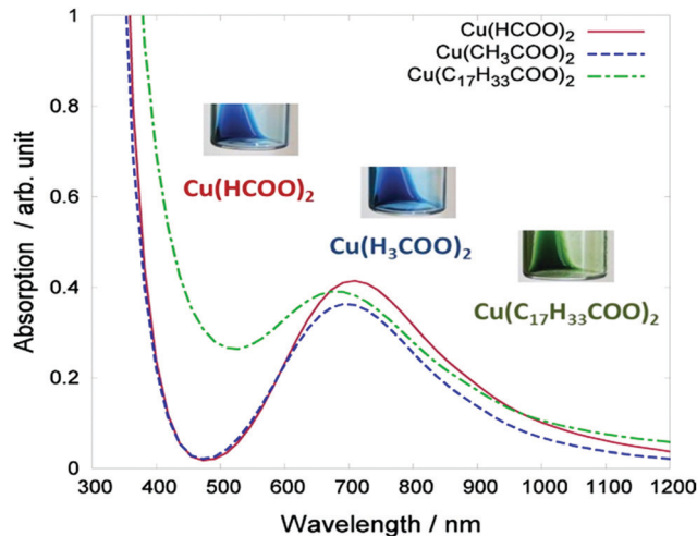
Fig. 7 Absorption spectra of the three types of copper complex ink: copper formate Cu(HCOO) 2 , copper acetate Cu(CH 3 COO) 2 , and copper oleate Cu(C 17 H 33 COO) 2 . The inset photographs display the visual color of the inks. Reproduced with permission from ref. 111. Copyright 2013, American Chemical Society.
