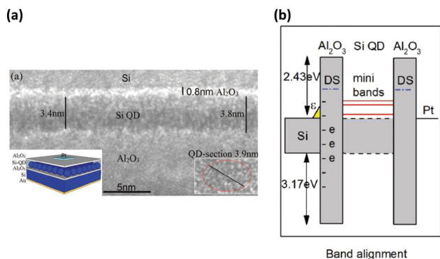
Fig. 2 TEM cross-section and sketch of an ESC based on silicon QDs (a). The QDs are sandwiched between thin layers of \text{Al}_2\text{O}_3 to form a double barrier resonant tunnelling structure. The sketch in (b) shows the involved energy levels with the discrete levels of Si QDs within the barrier. 26 Copyright 2017, published by Wiley-VCH.
