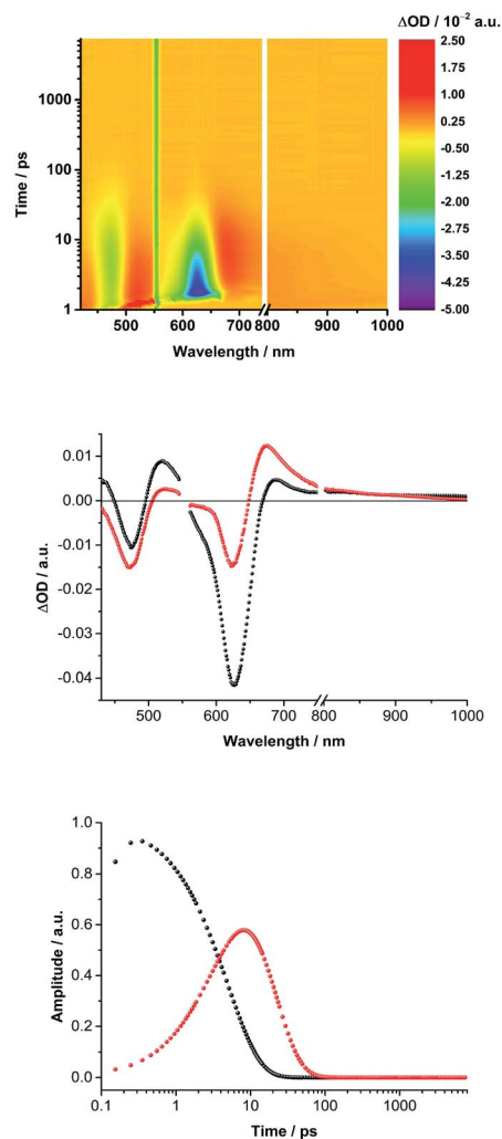
Fig. 4 (Top) Differential absorption spectra obtained by femtosecond transient absorption pump–probe experiments (550 nm, 400 nJ) of (TCBD-aniline) 3 -SubPc('BuPhO) 1 ( 2 \times 10^{-5} M) in argon-saturated anisole with several time delays between 1 to 7500 ps. (Middle) Deconvoluted evolution associated spectra and (bottom) associated time-dependent amplitudes obtained via global analysis in GloTarAn monitoring formation and decay kinetics.
