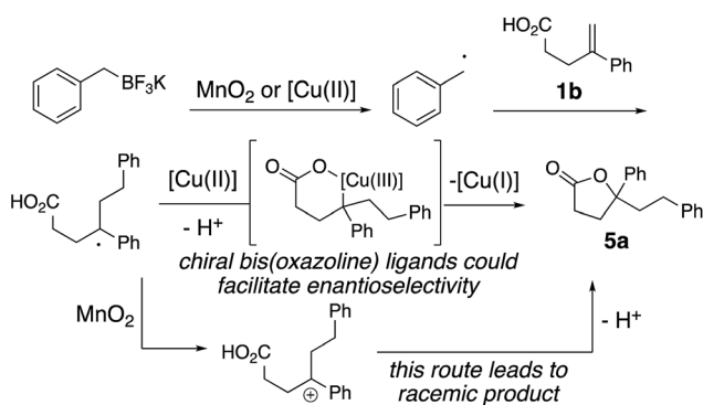
Scheme 3 Proposed mechanism.
