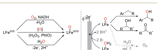
Scheme 1 Different approaches for the generation of high-valent iron-oxo species (left) and illustration of the application of electrochemical iron-oxo generation to the selective oxidation of organic molecules (right).
