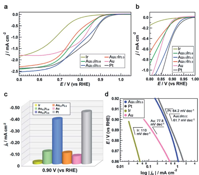
Fig. 5 Electrochemical oxygen-reduction activities of Au x Ir 1- x alloy catalysts. (a), (b) rotating disk electrode l - V polarization curves taken in O 2 -saturated 1.0 M NaOH aqueous solution normalized by the glassy carbon electrode geometric area (0.196 cm 2 ) from 0.50 to 1.05 V RHE and (b) from 0.80 to 1.00 V RHE . (c) Summary of the kinetic current densities for oxygen reduction on each catalyst measured at 0.90 V RHE . (d) Tafel plots for the catalysts. All of the NPs were loaded on carbon support.
