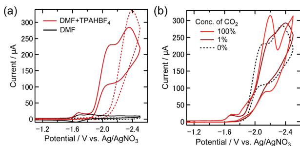
Fig. 7 (a) CVs of Re-DMF + (0.5 mM) in Ar-purged DMF with (red) and without (black line) 25 mM TPAHBF 4 as a proton source (dashed line: without Re-DMF + ). (b) CVs of Re-DMF + (0.5 mM) in the solution containing 100% CO 2 (red), 1% CO 2 (maroon line), and pure Ar (black dotted line). The solutions contain Et 4 NBF 4 (0.1 M) as the supporting electrolyte. The sweep rate was 200 mV s −1 . A glassy carbon electrode (diameter: 3 mm), an Ag/AgNO 3 (10 mM) electrode and a Pt wire were used as working, reference, and counter electrodes, respectively.
