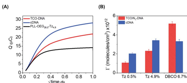
Fig. 4 (A) Example of CC curves measured for the gold electrodes modified with 0.25 \text{ mg mL}^{-1} of PLL-OEG(26.0)-Tz(4.9), 1 \text{ }\mu\text{M} TCO-DNA and cDNA in the presence of 50 \text{ }\mu\text{M} RuHex in 20 \text{ mM} Tris buffer. (B) Surface coverage of Au electrode surfaces modified with PLL-OEG-Tz(0.5), PLL-OEG-Tz(4.9) and PLL-OEG-DBCO(6.7) and subsequently with TCO-DNA and \text{N}_3 -DNA, before and after hybridization with cDNA.
