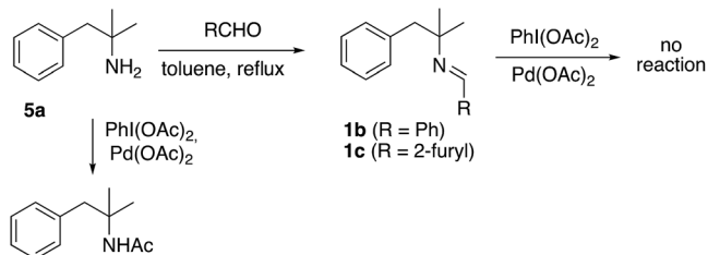
Scheme 3 Alternative nitrogen atoms as directing groups.
