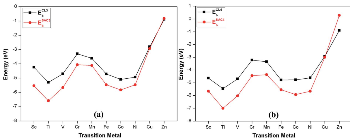
Fig. 2 E_b^{SAC3} and E_b^{SAC4} are the binding energies of embedded three and four metal atoms with the B_{812} monolayer. E_b^{CL3} and E_b^{CL4} are the binding energies of metal clusters (comprised of three and four metal atoms) with the B_{812} monolayer.
