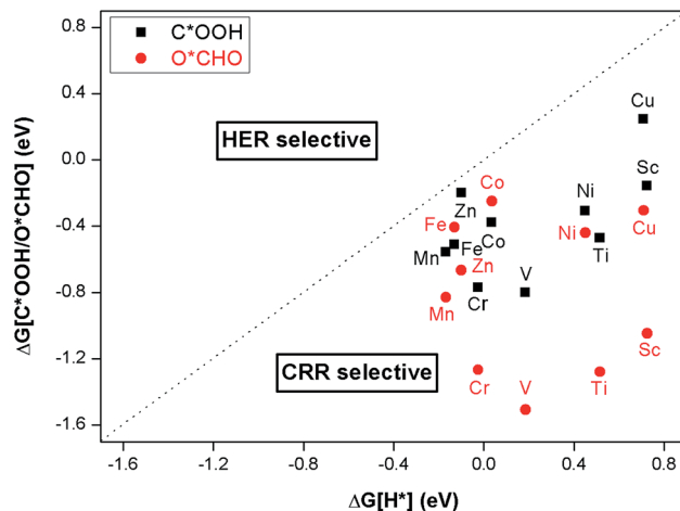
Fig. 3 \Delta G_{\text{COOH}^*} and \Delta G_{\text{OCHO}^*} are the Gibbs free energy change of the first protonation step in CRR and \Delta G_{\text{H}^*} is for HER. Catalysts below the dotted line are CRR selective.
