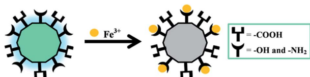
Scheme 2 Schematic illustration of a possible fluorescence-quenching mechanism.
