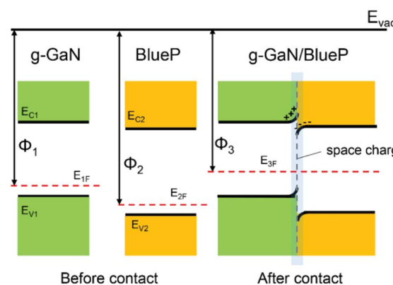
Fig. 6 Energy-band diagrams of BlueP and g-GaN; schematic diagram of vdW heterostructure of BlueP and g-GaN.
