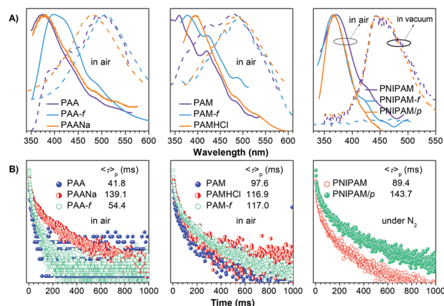
Fig. 4 (A) Emission spectra with t_{\text{d}} of 0 (solid line) and 0.1 ms (dash line) and (B) RTP decay curves of different films (f) and powders in air, under nitrogen, or in vacuum. Detailed \lambda_{\text{ex}} s for the emission measurement and monitored wavelengths for the lifetime test are listed in Tables S1 and S2 (ESI†).
