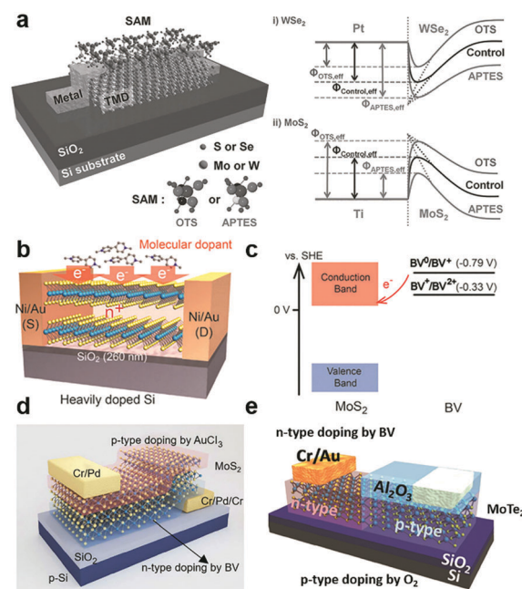
Fig. 8 Charge transfer doping of 2D MXs by organic small molecules: (a) SAM to modulate the interfacial Schottky barrier for electrical contact to 2D TMDs, reprinted with permission from ref. 142, Copyright 2015 Wiley-VCH. (b) Reductive n-type doping of \text{MoS}_2 by BV molecules and (c) the related redox processes, reprinted with permission from ref. 126, Copyright 2014 American Chemical Society. (d) Vertical and (e) lateral PN junctions enabled by combined BV induced doping and other doping methods, reprinted with permission from ref. 162, Copyright 2015 Nature publishing group, and ref. 150 Copyright 2017 Wiley-VCH.
