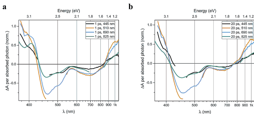
Fig. 4 Transient absorption spectra of Fe II (btz) 3 at (a) 1 ps, and (b) 20 ps normalized by the number of absorbed photons per cm 2 at each respective excitation wavelength. The x-axis (wavelength) is in reciprocal values (linear steps in energy).
