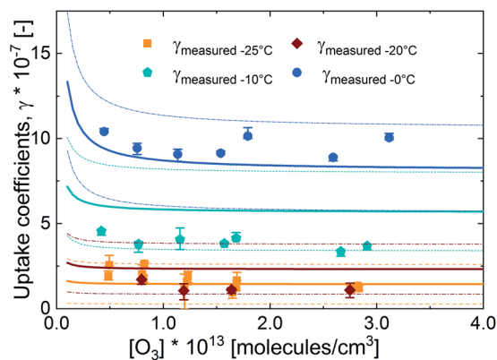
Fig. 6 Measured and parameterized uptake coefficients ( H_{\text{O}_3\text{Mix\_CA}\text{salt-in(T-ind)}} ) with error bands at different temperatures as a function of gas-phase ozone concentration. The dots are the measured uptake coefficients; the solid lines are the model lines; the thin dashed lines are the error bands for the parameterization output. The parameterization output and error bands have the same colour as the temperature in question: blue circles ● for 0 °C, cyan pentagons ◆ for −10 °C, red diamonds ◆ for −20 °C, and orange squares ■ for −25 °C.
