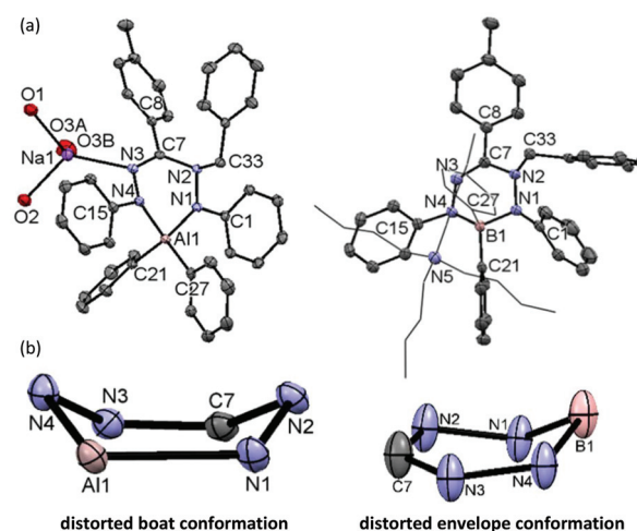
Fig. 2 (a) Molecular structures of [ \text{B}^{\text{Bn}2} ][Na] (top, left) and [ \text{B}^{\text{Bn}1} ][NBu 4 ] (top, right), showing 50% probability ellipsoids. Hydrogen atoms for [ \text{B}^{\text{Bn}2} ][Na] and [ \text{B}^{\text{Bn}1} ][NBu 4 ] are omitted for clarity. THF molecules (except for the O atoms bonded to Na) are omitted for clarity. (b) Six-membered chelate rings for [ \text{B}^{\text{Bn}2} ][Na] (bottom, left) and for [ \text{B}^{\text{Bn}1} ][NBu 4 ] (bottom, right).
