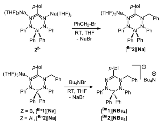
Scheme 2 Synthesis of ligand-benzylated products [ \text{B}^{\text{Bn}2} ][Na], [ \text{B}^{\text{Bn}2} ][NBu 4 ] and [ \text{B}^{\text{Bn}1} ][NBu 4 ].
