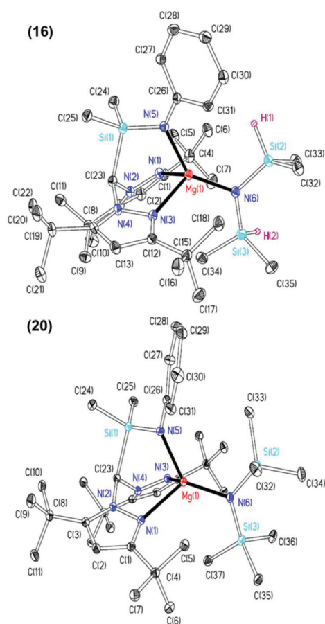
Fig. 2 Thermal displacement ellipsoid drawings (20% probability ellipsoids) of Mg\{HC(iBu_2pz)_2SiMe_2NPh\}\{N(SiHMe_2)_2\} ( 16 , top) and Mg\{HC(iBu_2pz)_2SiMe_2NPh\}\{N(SiMe_3)_2\} ( 20 , bottom). C-Bound hydrogen atoms have been omitted for clarity.
