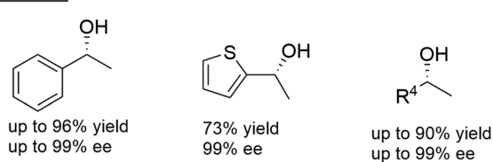
Scheme 8 Examples for CD-OS of alcohols using Gardenia jasminoides or Geotrichum candidum as KR catalysts coupled to non-selective reduction of the intermediate ketone by \text{NaBH}_4 .
