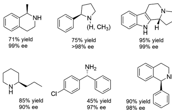
Scheme 9 Cyclic deracemisation via stereospecific oxidative step (CD-OS) of amines using monoamine oxidase (MAO-N, EC:1.4.3.4) and its variants together with \text{NH}_3\text{BH}_3 as a stoichiometric, non-stereoselective reductant.
