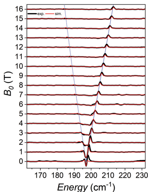
Fig. 2 THz-EPR spectra for a fine-crystalline sample of CoTp 2 at 4.2 K (black). MDS spectra at the magnetic field B_0 are obtained by dividing a spectrum measured at B_0 by a spectrum measured at B_0 + 1 T; data is offset for B_0 . Simulation with the spin-Hamiltonian (1) ( S = 3/2 , D = -98.5 cm -1 , g_{\perp} = 1.9 , g_{\parallel} = 2.1 ) is shown in red. Blue lines correspond to the transition energies for B_0 perpendicular (dashed) and parallel (solid) to the molecular easy axis.
