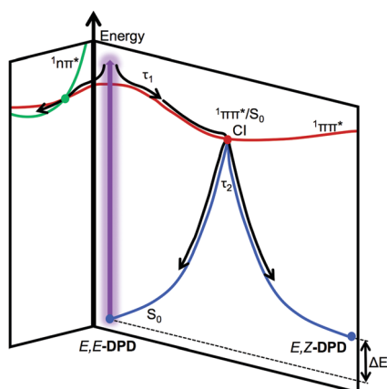
Fig. 3 Schematic of relaxation for photoexcited E,E -DPD, showing the progression of \tau_1 and \tau_2 . We add that \tau_3 (not shown) would correspond to population trapped in the E,Z -DPD and 1n\pi^* state.
