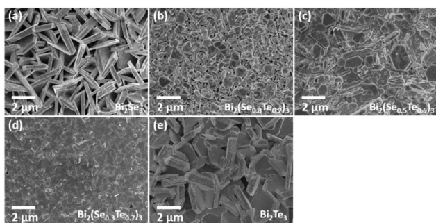
Fig. 3 SEM images showing the morphologies of the \text{Bi}_2\text{Se}_3 (a), \text{Bi}_2\text{Te}_3 (e) and ternary \text{Bi}_2(\text{Se}_{1-x}\text{Te}_x)_3 (b–d) films deposited by LPCVD under similar conditions (550 ^\circ\text{C} /0.05 mmHg) onto \text{SiO}_2 -coated silicon substrates.
