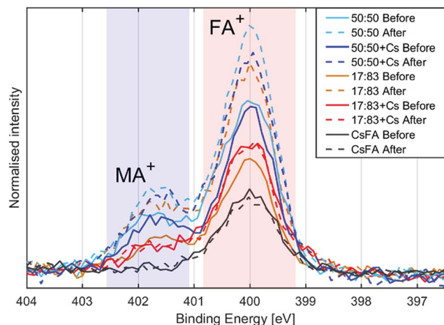
Fig. 6 N1s spectra of the different compositions before and after illumination, normalised to \text{Pb}(+\text{II}) 4f intensity and aligned with peak maximum at 400 eV.
